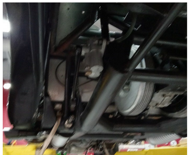
Old Jaguar AGS with inboard rear brakes
